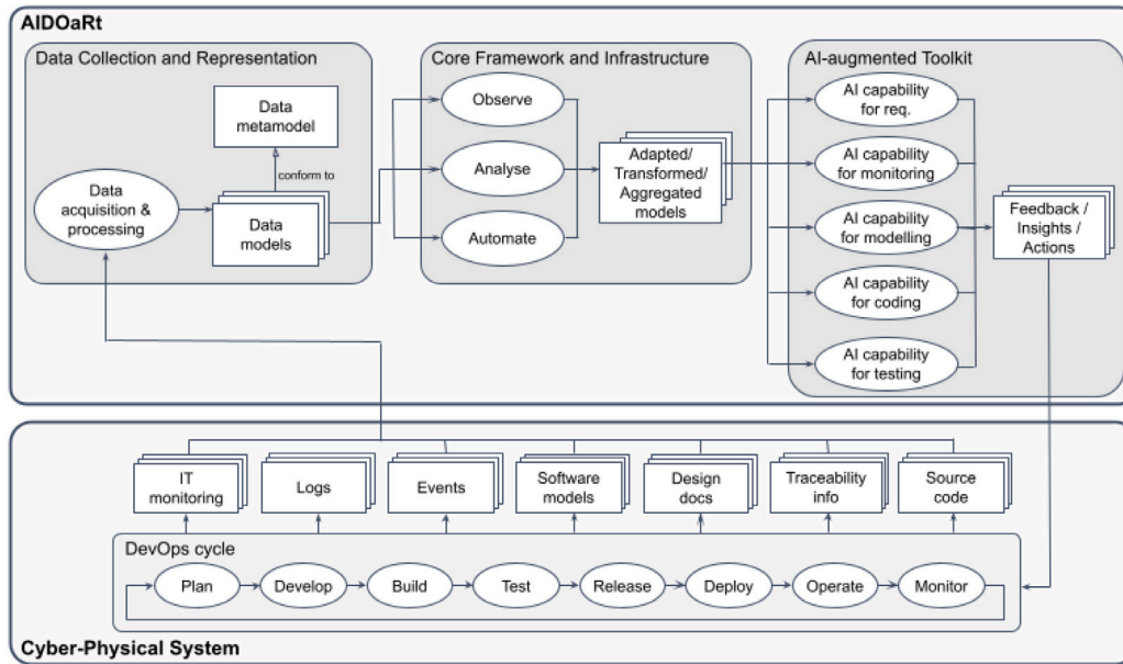
Fig. 3. AIDOaRt approach.
