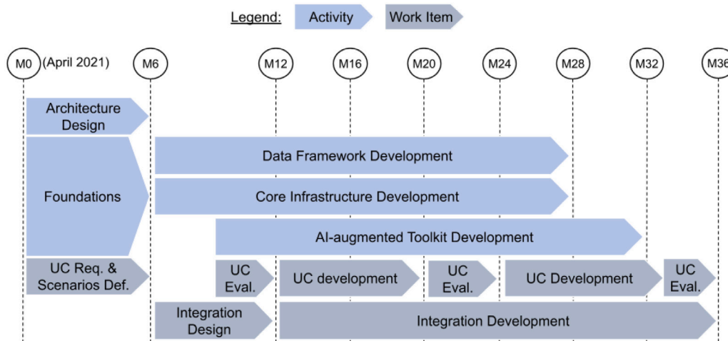
Fig. 5. AIDOaRt timeline.
